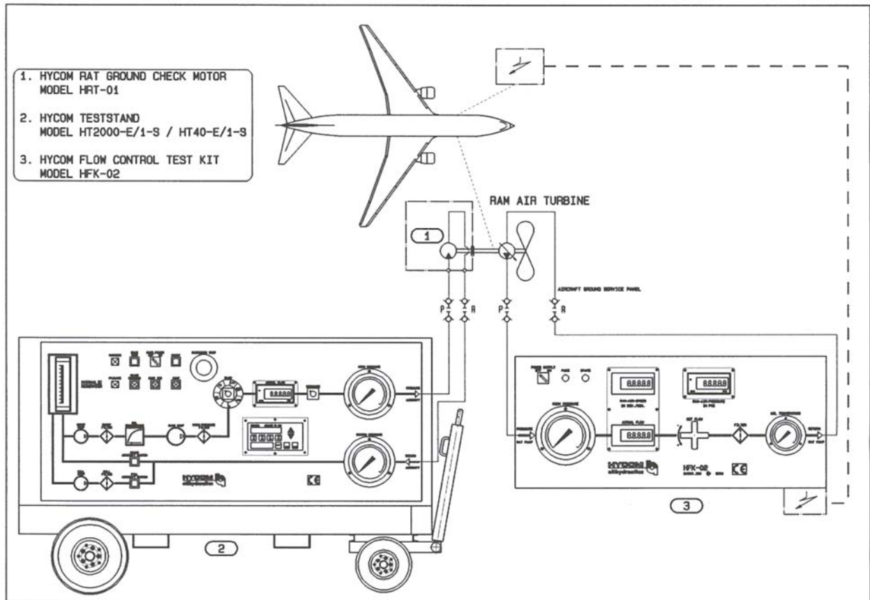
HFK02 Flow control test kit and checkout unit
