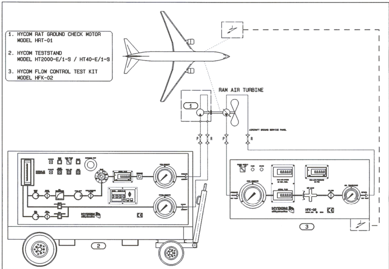
HFK02 Flow control test kit and checkout unit HRK01 is the order code for the complete test kit consisting of HFK02 and HRT01.
